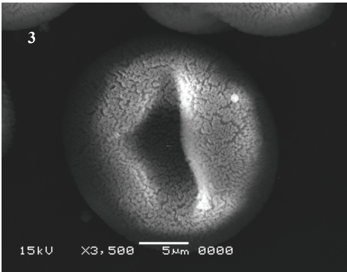
Plate VI. Spores of Entosthodon muhlenbergii with SEM. 1–5, 1-group of spores, leptoma is longitudinal, 2-Distal view of elliptic spore, The ornamentation is baculate, 3-Proximal view of a spore with longitudinal leptoma, the ornamentation is baculate, 4-Equatorial view of a concave-hemispheric spore, the surface near the leptoma is psilate, 5-Detail of the baculate distal surface, bacula are long, dense and tapering.
