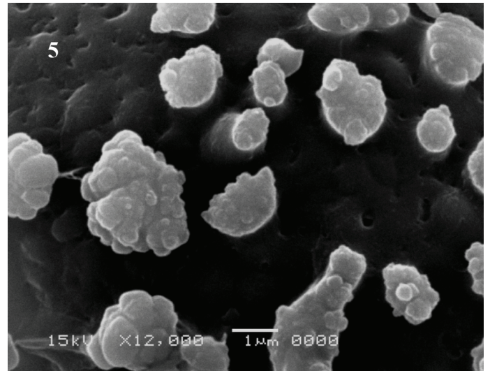
Plate VII. Spores of Entosthodon attenuatus with SEM. 1–5, 1-Distal to equatorial view of convex- hemispherical spore, the ornamentation is clavate- foveolate, 2-Proximal view of a spore with rounded leptoma, the ornamentation is clavate- foveolate, 3-Equatorial view of concave- hemispherical spore, 4-detail of equatorial view of spore, 5-Detail of the clavate- foveolate distal surface. Clavae elements are irregular in size.
