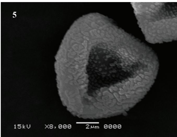
Plate IV. Spores of Tortula mularis with SEM. 1–5.1-Group of spores, leptoma is triangular, 2- Distal view of semi-spherical spore. The ornamentation is regulate, 3-Proximal view of a spore with a triangular leptoma, The ornamentation is regulate, 4-Equatorial view of a concave-hemispheric spore, 5-Detail of the rugulate distal surface, The ridges are irregular and are fused to one another.
