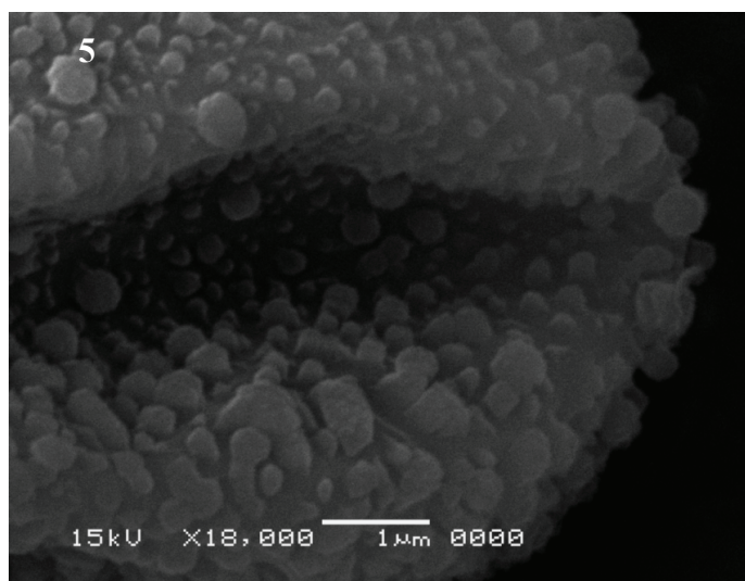
Plate VIII. Spores of Funaria hygrometrica with SEM. 1–5, 1-Distal view of semi-spherical spore, the ornamentation is clavate, 2-Proximal view of a spore with quadrangular leptoma, the ornamentation is verrucate, 3-Proximal view of a spore with longitudinal leptoma, the ornamentation is verrucate, 4-Equatorial view of a concave-hemispheric spore, 5-Detail of the verrucate-gemmate proximal surface, verrucae are irregular in size.
