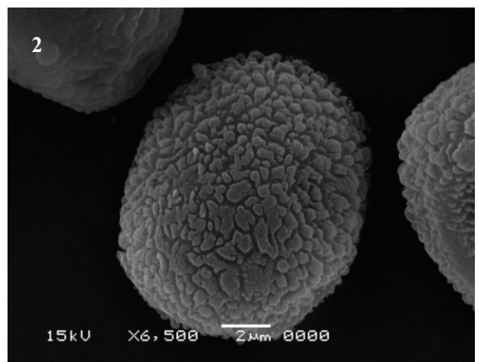
Plate II. Spores of Microbryum davallianum with SEM. 1–4, 1-Distal view of semi-spherical spore, the ornamentation is foveolate- psilate, 2-Distal view of semi-spherical spore, the ornamentation is rugulate with foveolae, 3-Proximal view of a spore with triangular leptoma, the surface near the leptoma is psilate. A globule located on a foveola can be observed (arrow), 4- Detail of the rugulate- foveolate distal surface.
