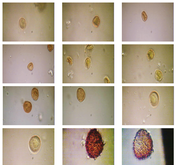
Plate IX. Spores by light microscope a-l (a,b: Aloina brevirostris ; c,d: Tortula mularis ; e,f: Tortula brevissima ; g,h: Entosthodon muhlenbergii ; i,j: Funaria hygrometrica ; k,l: Entosthodon attenuates , all figs., X: 1000
