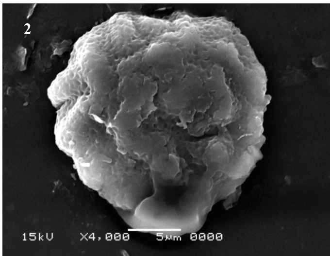
Plate II. Spores of Microbryum davallianum with SEM. 1–4, 1-Distal view of semi-spherical spore, the ornamentation is foveolate- psilate, 2-Distal view of semi-spherical spore, the ornamentation is rugulate with foveolae, 3-Proximal view of a spore with triangular leptoma, the surface near the leptoma is psilate. A globule located on a foveola can be observed (arrow), 4- Detail of the rugulate- foveolate distal surface.
