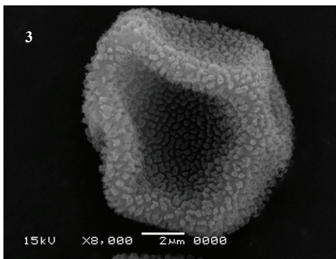
Plate I. Spores of Aloina brevirostris with SEM. 1–5, 1-Group of quinquangular spores, leptoma is triangular, elliptic, 2-Distal view of semi-spherical spore, the ornamentation is piloid, 3-Proximal view of a spore with pentagonal leptoma. the ornamentation is piloid, 4-Equatorial view of elliptic spore, 5-Detail of the piloid distal surface.
