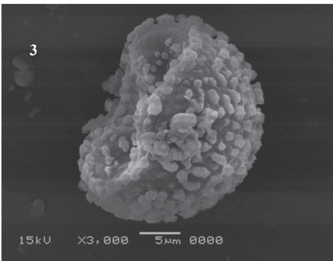
Plate VII. Spores of Entosthodon attenuatus with SEM. 1–5, 1-Distal to equatorial view of convex- hemispherical spore, the ornamentation is clavate- foveolate, 2-Proximal view of a spore with rounded leptoma, the ornamentation is clavate- foveolate, 3-Equatorial view of concave- hemispherical spore, 4-detail of equatorial view of spore, 5-Detail of the clavate- foveolate distal surface. Clavae elements are irregular in size.
