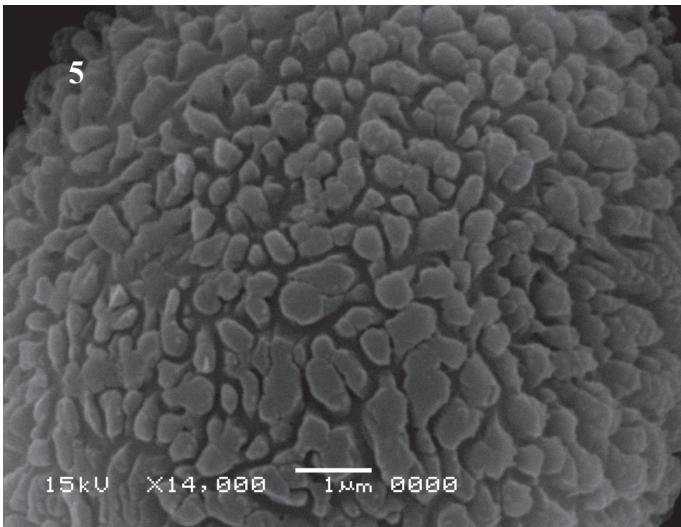
Plate III. Spores of Syntrichia laevipila with SEM. 1–5, 1-Group of spores, leptoma is elliptic, 2- Distal view of subprolate spore, the ornamentation is verrucate- regulate, 3-Proximal view of a spore with elliptic leptoma, the ornamentation is granulate, 4-Equatorial view of a concave-hemispheric spore, the surface near the leptoma is psilate, 5-Detail of the verrucate- rugulate distal surface, the muri are irregular in thickness
