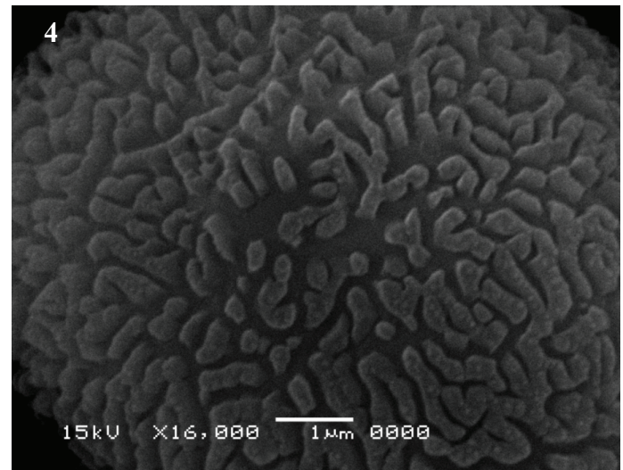
Plate IV. Spores of Tortula mularis with SEM. 1–5.1-Group of spores, leptoma is triangular, 2- Distal view of semi-spherical spore. The ornamentation is regulate, 3-Proximal view of a spore with a triangular leptoma, The ornamentation is regulate, 4-Equatorial view of a concave-hemispheric spore, 5-Detail of the rugulate distal surface, The ridges are irregular and are fused to one another.
