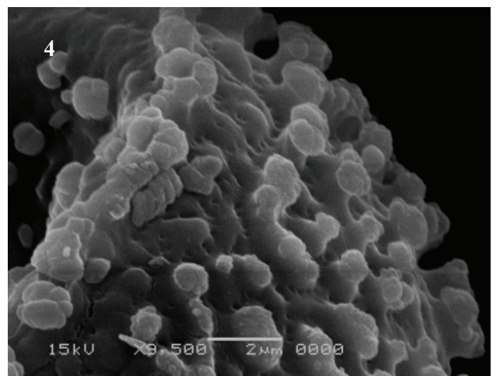
Plate VI. Spores of Entosthodon muhlenbergii with SEM. 1–5, 1-group of spores, leptoma is longitudinal, 2-Distal view of elliptic spore, The ornamentation is baculate, 3-Proximal view of a spore with longitudinal leptoma, the ornamentation is baculate, 4-Equatorial view of a concave-hemispheric spore, the surface near the leptoma is psilate, 5-Detail of the baculate distal surface, bacula are long, dense and tapering.
