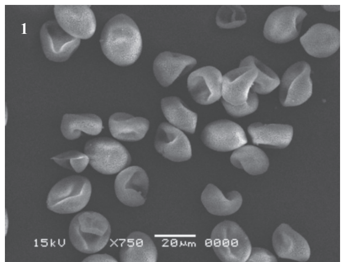
Plate V. Spores of Tortula brevissima with SEM. 1–5, 1-Group of spores, leptoma is rounded, triangular, 2-Distal view of semi-spherical spore, the ornamentation is verrucate- regulate, 3-Proximal view of a spore with rounded to triangular leptoma, the ornamentation is verrucate- granulate, 4-Equatorial view of a concave-hemispheric spore, the surface near the leptoma is psilate, 5-Detail of the verrucate- granulate proximal surface.
