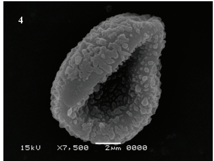
Plate III. Spores of Syntrichia laevipila with SEM. 1–5, 1-Group of spores, leptoma is elliptic, 2- Distal view of subprolate spore, the ornamentation is verrucate- regulate, 3-Proximal view of a spore with elliptic leptoma, the ornamentation is granulate, 4-Equatorial view of a concave-hemispheric spore, the surface near the leptoma is psilate, 5-Detail of the verrucate- rugulate distal surface, the muri are irregular in thickness
